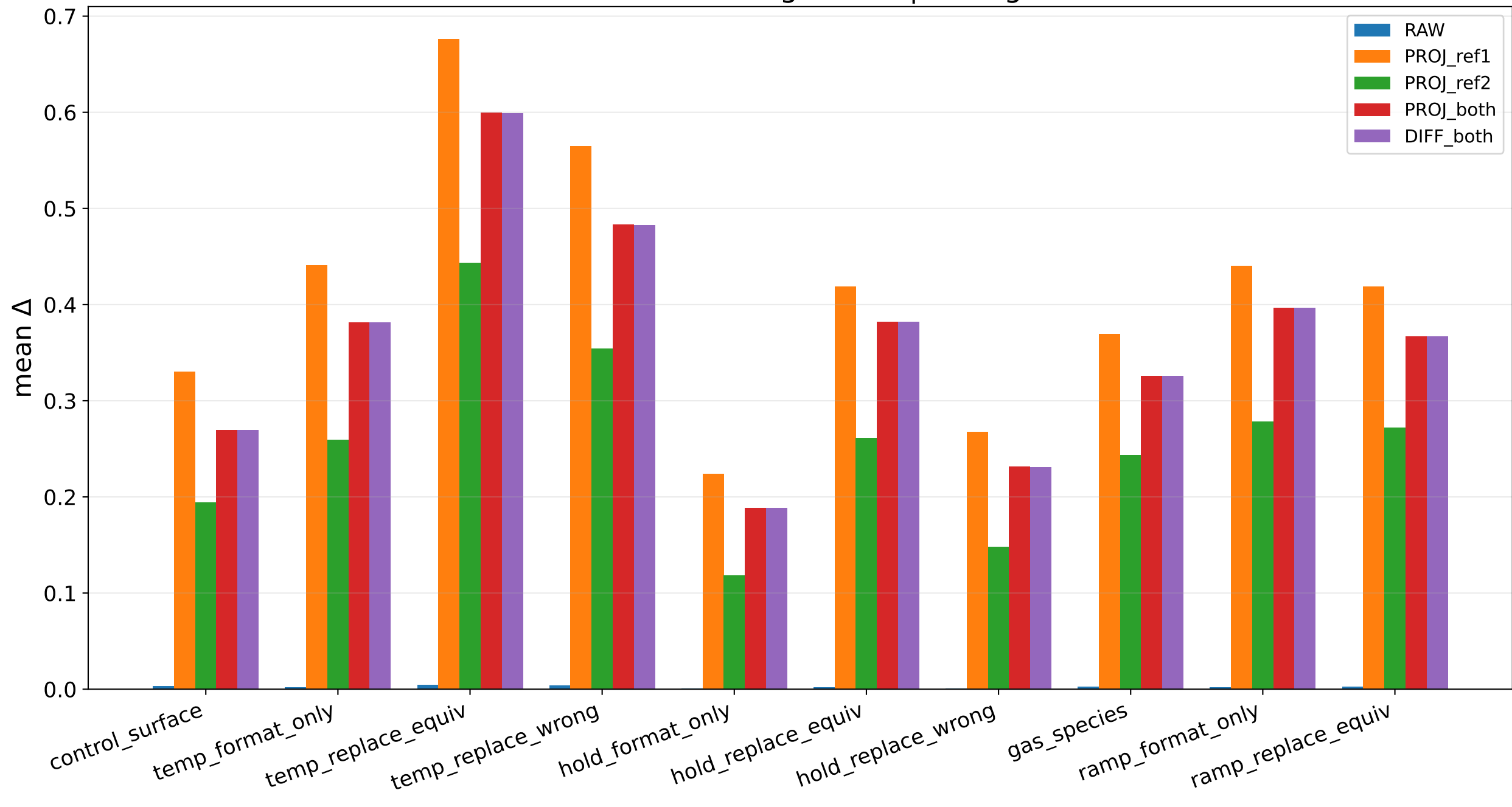
Effect of scoring mode | 3-large
